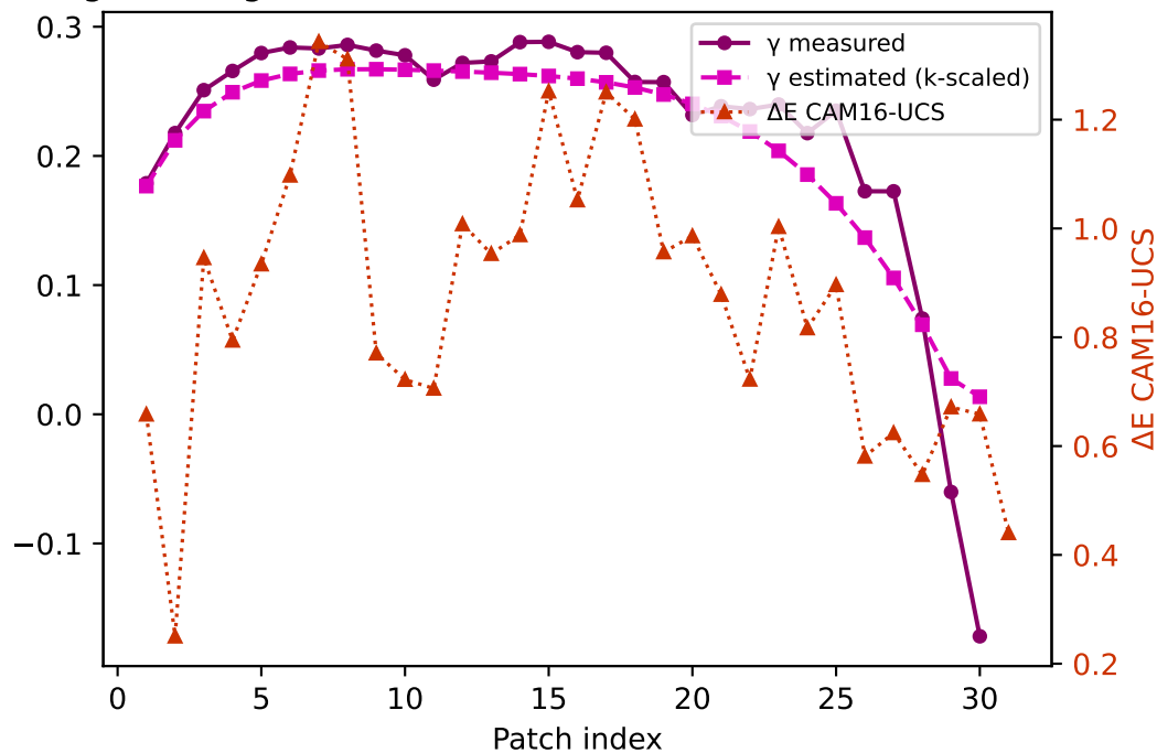
Magenta — gamma k=0.8955 mean \Delta E=0.872 std=0.256
