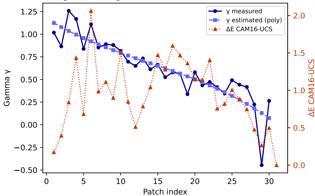
B — gamma (degree 3) mean \Delta E=0.954 std=0.456
