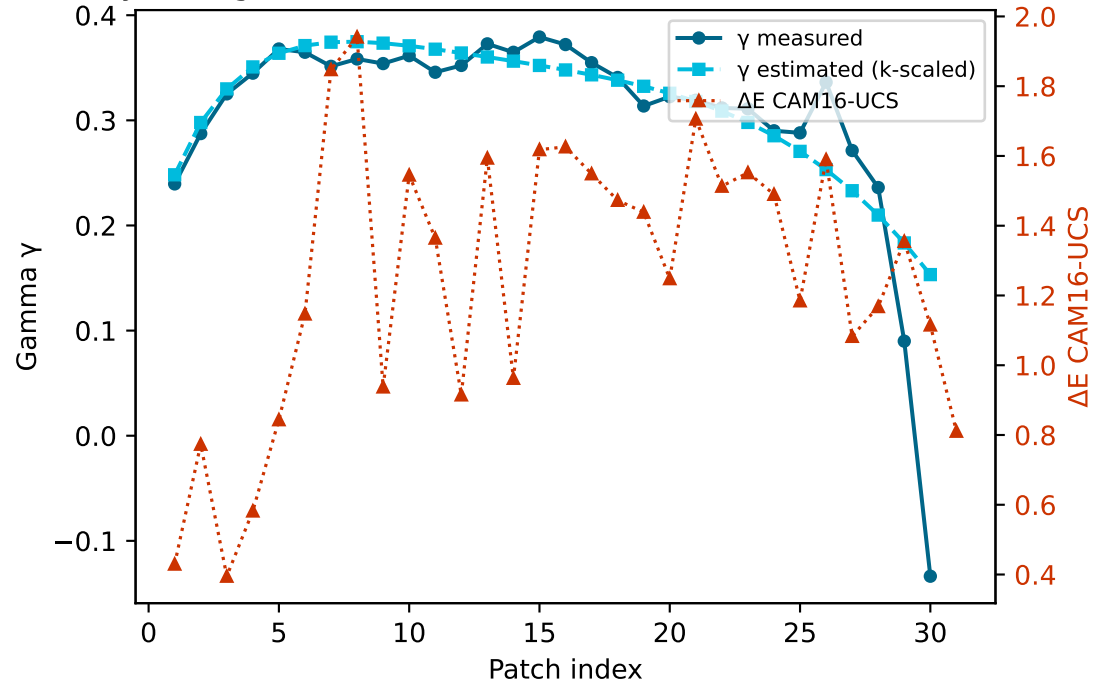
Gray — gamma k=0.9529 mean \Delta E=1.535 std=0.666
